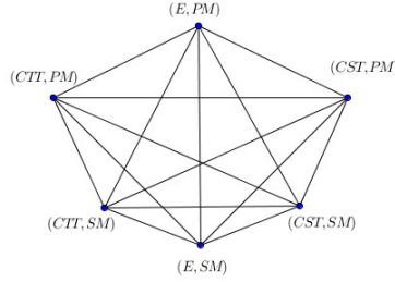
Figure 7: Vague graph G_1[G_2]_{min}^v and G_1[G_2]_{max}^v
