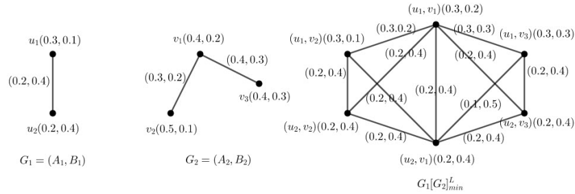
Figure 3: Vague graph G_1 , G_2 and G_1[G_2]_{min}^L
