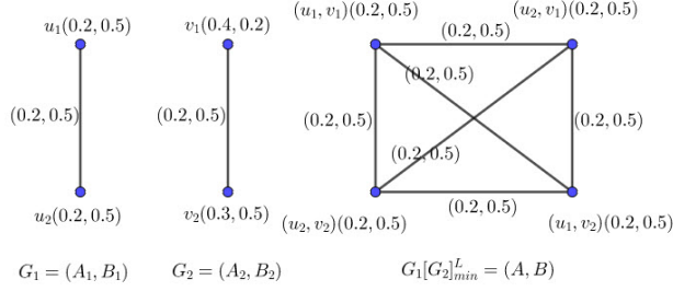
Figure 4: Vague graph G_1 , G_2 and G_1[G_2]_{min}^L
