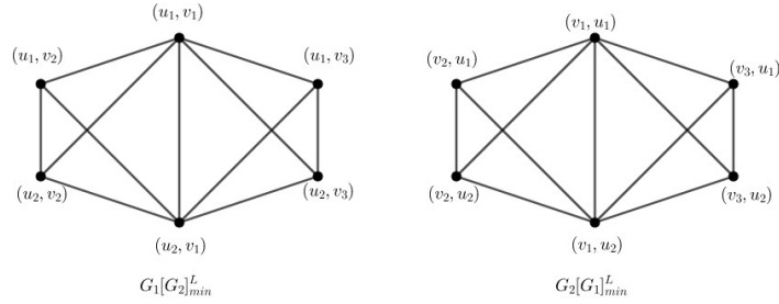
Figure 2: Vague graphs G_1[G_2]_{min}^L and G_2[G_1]_{min}^L
