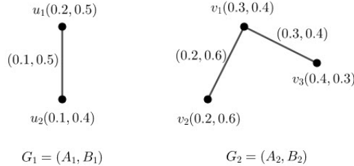
Figure 1: Vague graphs G_1 and G_2
