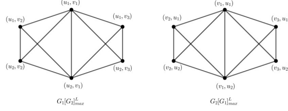
Figure 5: Vague graphs G_1[G_2]_{max}^L and G_2[G_1]_{max}^L
