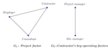
Figure 6: Vague graphs G_1 and G_2
